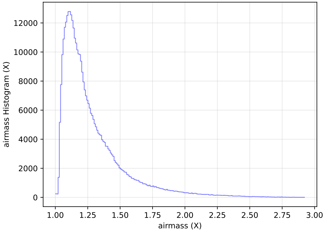
too_elab_heavy_r64_d2_ugrizy_v3.4_10yrs WFD y band: airmass Histogram
