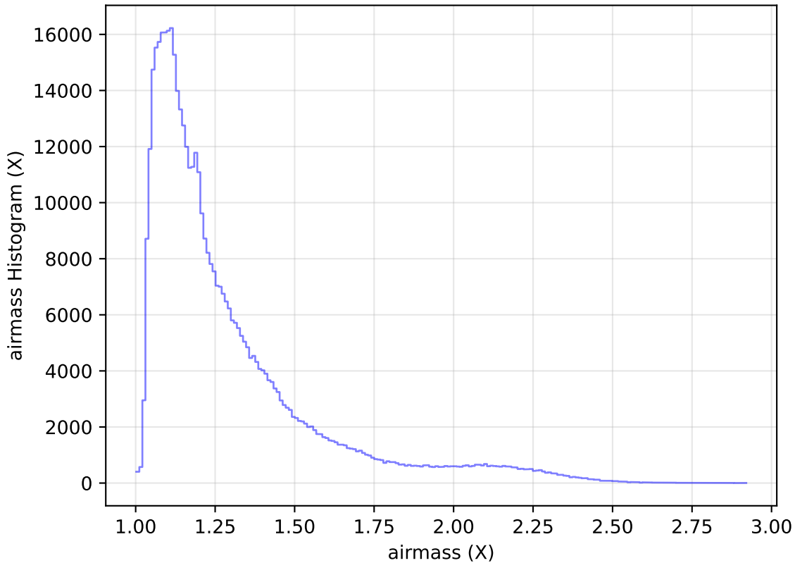
too_elab_heavy_r64_d2_ugrizy_v3.4_10yrs WFD r band: airmass Histogram
