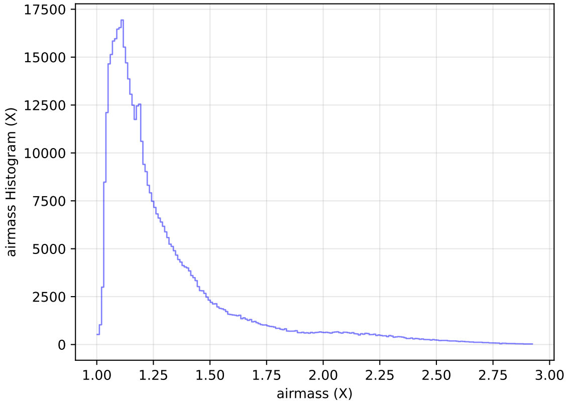
too_elab_heavy_r64_d2_ugrizy_v3.4_10yrs WFD i band: airmass Histogram
