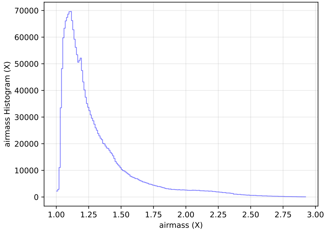
too_elab_heavy_r64_d2_ugrizy_v3.4_10yrs WFD all bands: airmass Histogram
