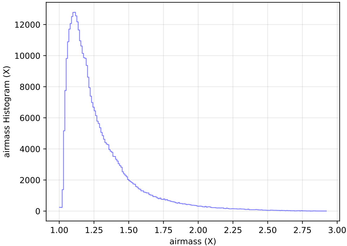
too_elab_heavy_r64_d2_ugrizy_v3.4_10yrs All sky y band: airmass Histogram
