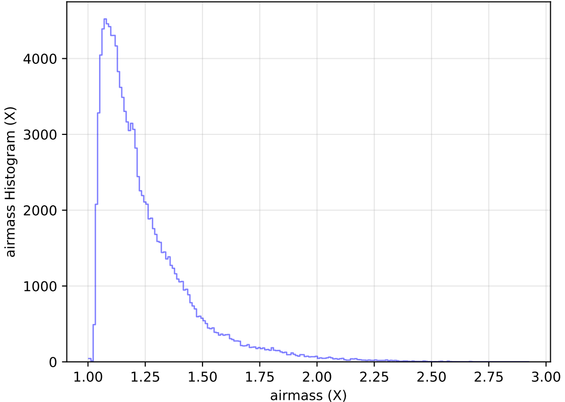
too_elab_heavy_r64_d2_ugrizy_v3.4_10yrs All sky u band: airmass Histogram
