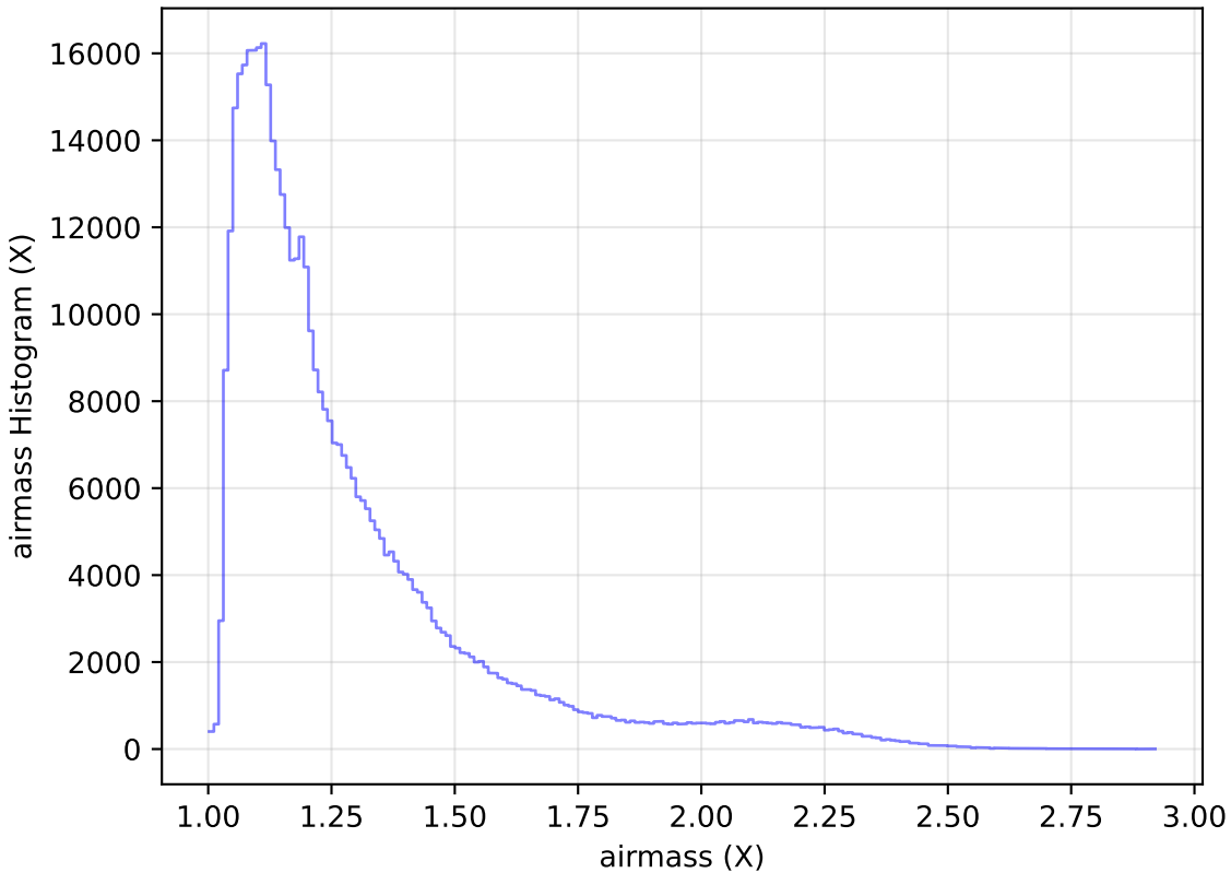
too_elab_heavy_r64_d2_ugrizy_v3.4_10yrs All sky r band: airmass Histogram
