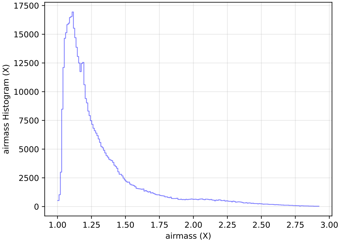
too_elab_heavy_r64_d2_ugrizy_v3.4_10yrs All sky i band: airmass Histogram
