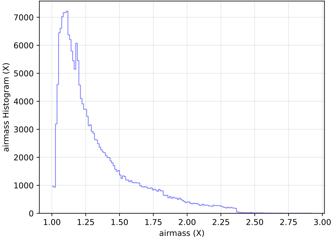
too_elab_heavy_r64_d2_ugrizy_v3.4_10yrs All sky g band: airmass Histogram
