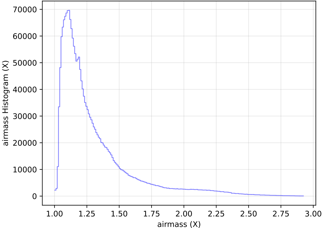
too_elab_heavy_r64_d2_ugrizy_v3.4_10yrs All sky all bands: airmass Histogram
