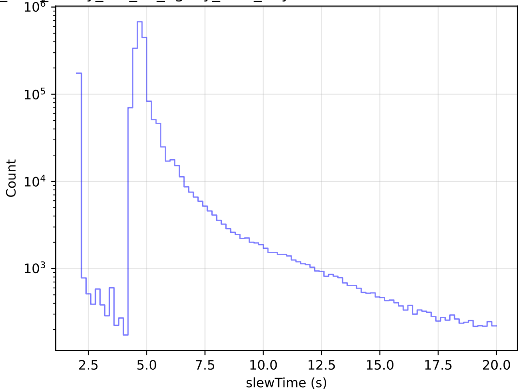
too_elab_heavy_r64_d2_ugrizy_v3.4_10yrs All visits: Zoom Slew Time Histogram
