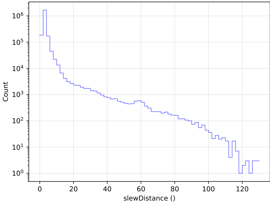
too_elab_heavy_r64_d2_ugrizy_v3.4_10yrs All visits: Slew Distance Histogram
