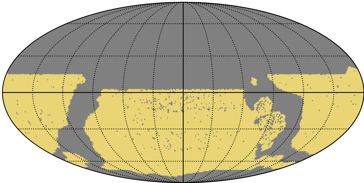
too_elab_heavy_r64_d2_ugrizy_v3.4_10yrs WFD: RapidRevisits
