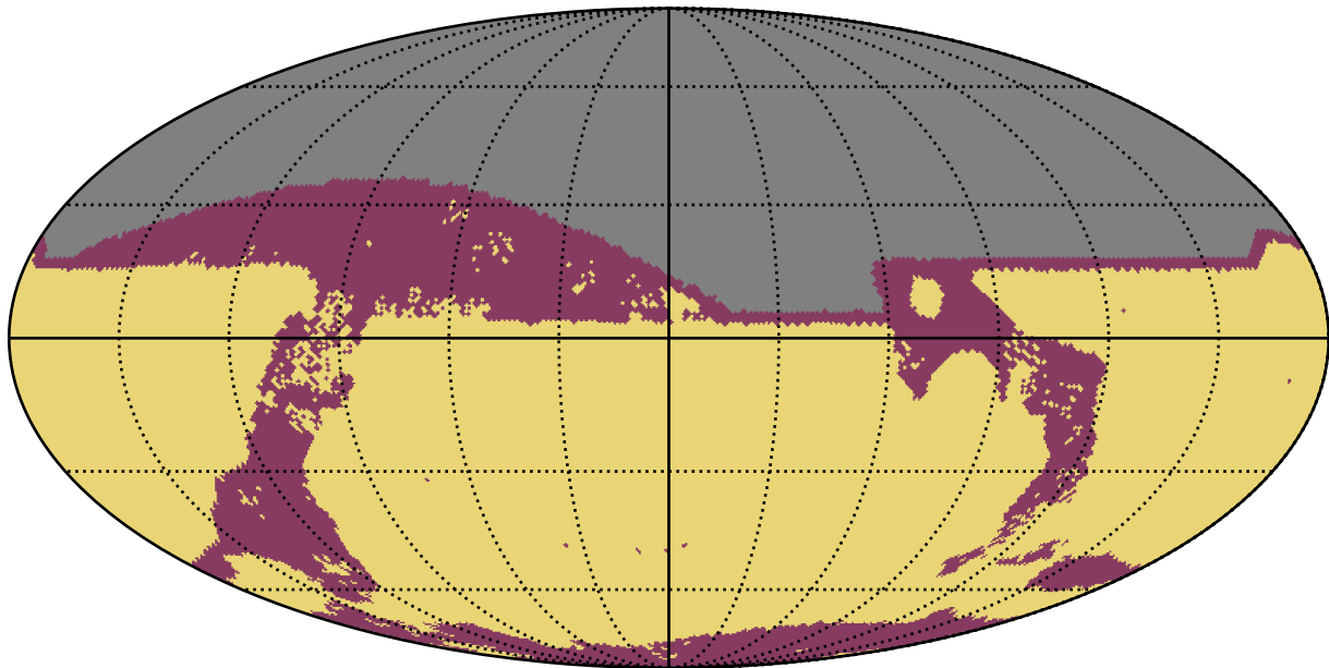
too_elab_heavy_r64_d2_ugrizy_v3.4_10yrs All sky: RapidRevisits
