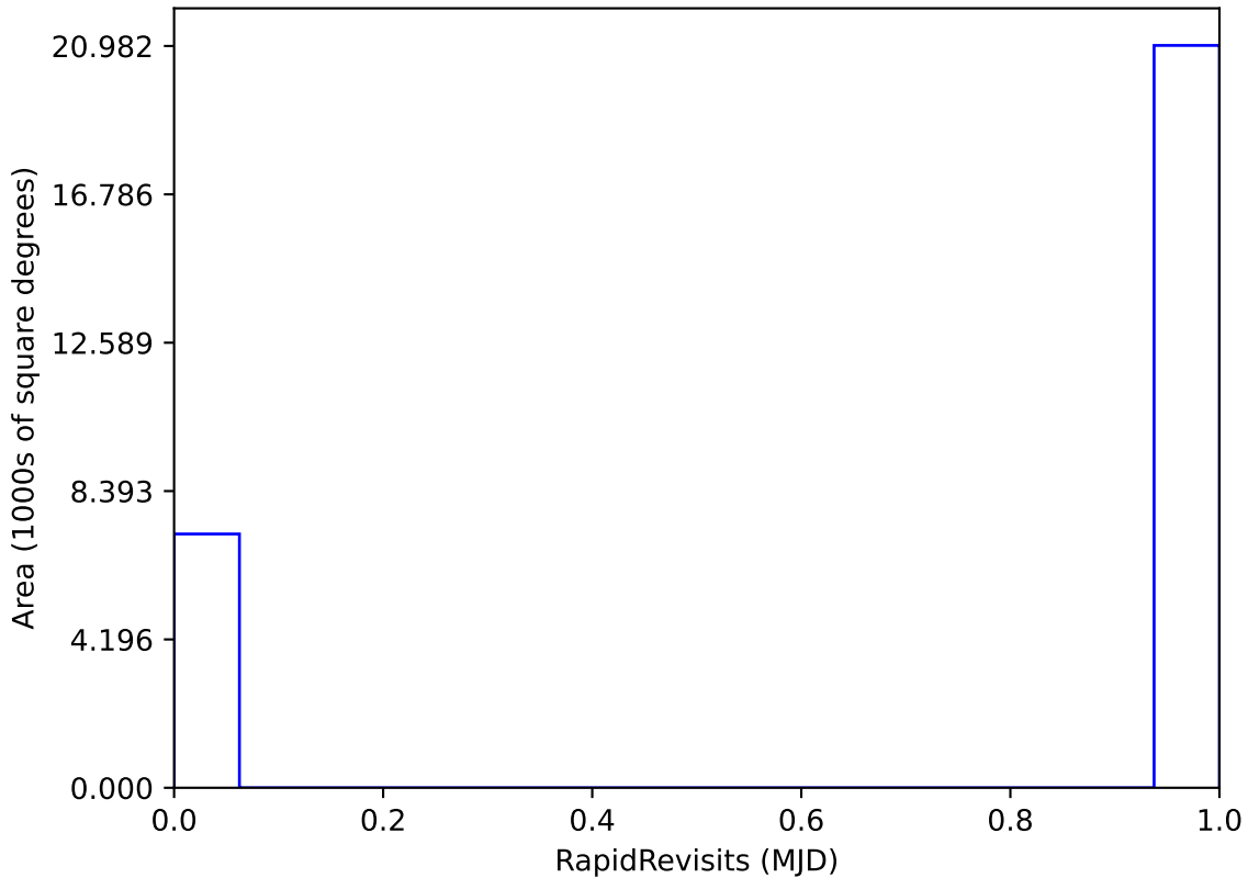
too_elab_heavy_r64_d2_ugrizy_v3.4_10yrs All sky: RapidRevisits
