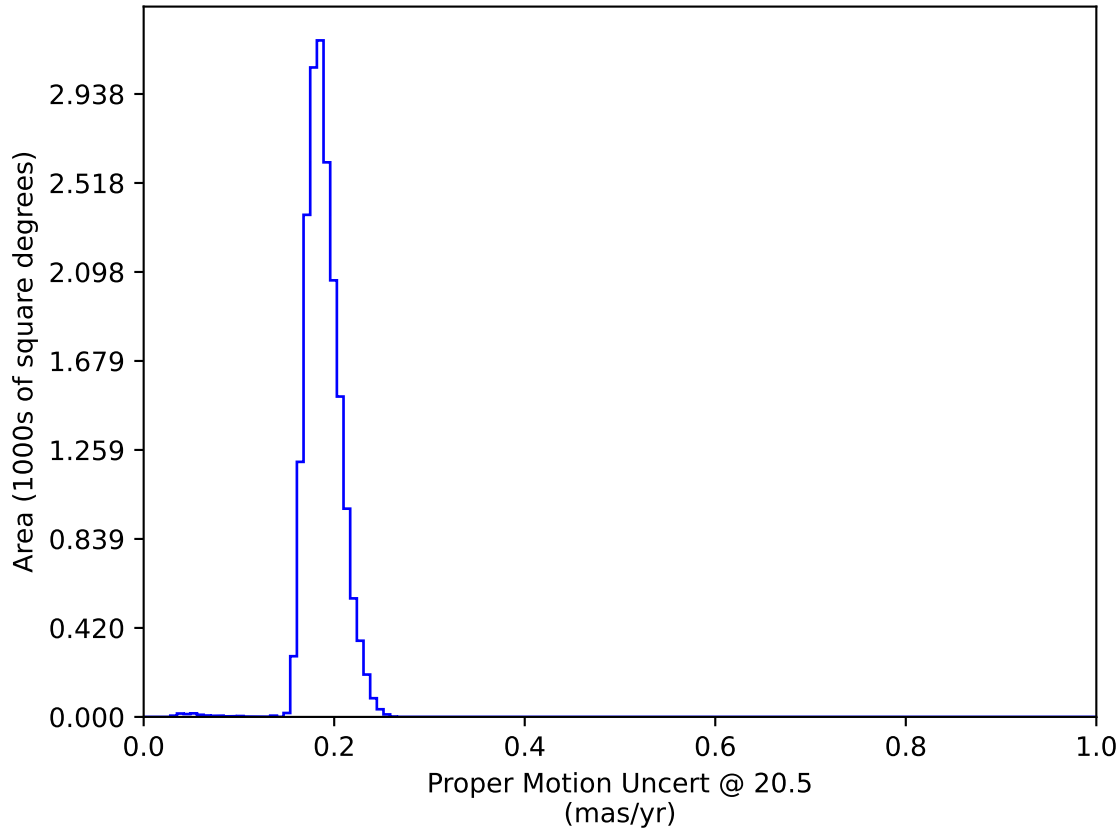
too_elab_heavy_r64_d2_ugrizy_v3.4_10yrs WFD: Proper Motion Uncert @ 20.5
