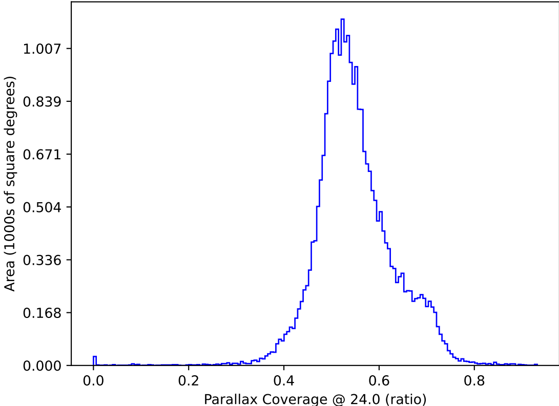
too_elab_heavy_r64_d2_ugrizy_v3.4_10yrs All sky: Parallax Coverage @ 24.0
