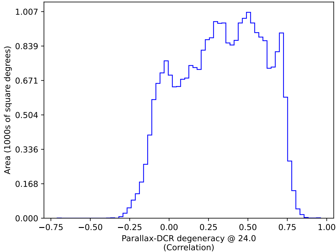
too_elab_heavy_r64_d2_ugrizy_v3.4_10yrs All sky: Parallax-DCR degeneracy @ 24.0
