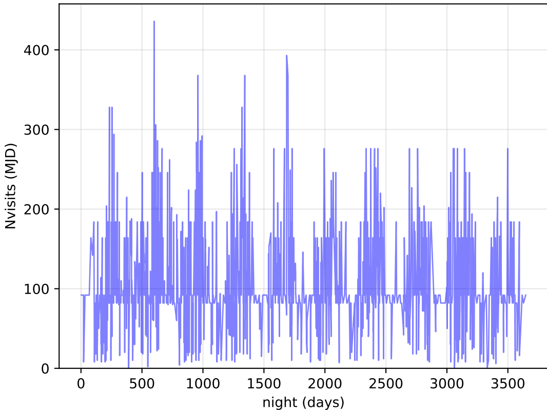
too_elab_heavy_r64_d2_ugrizy_v3.4_10yrs DDF: Nvisits
