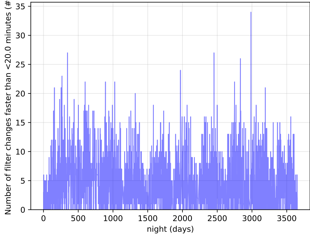
too_elab_heavy_r64_d2_ugrizy_v3.4_10yrs Per Night: Number of filter changes faster than <20.0 minutes
