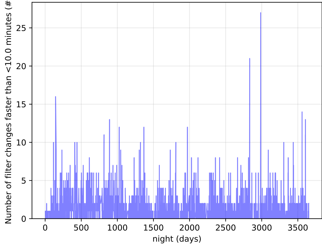
too_elab_heavy_r64_d2_ugrizy_v3.4_10yrs Per Night: Number of filter changes faster than <10.0 minutes
