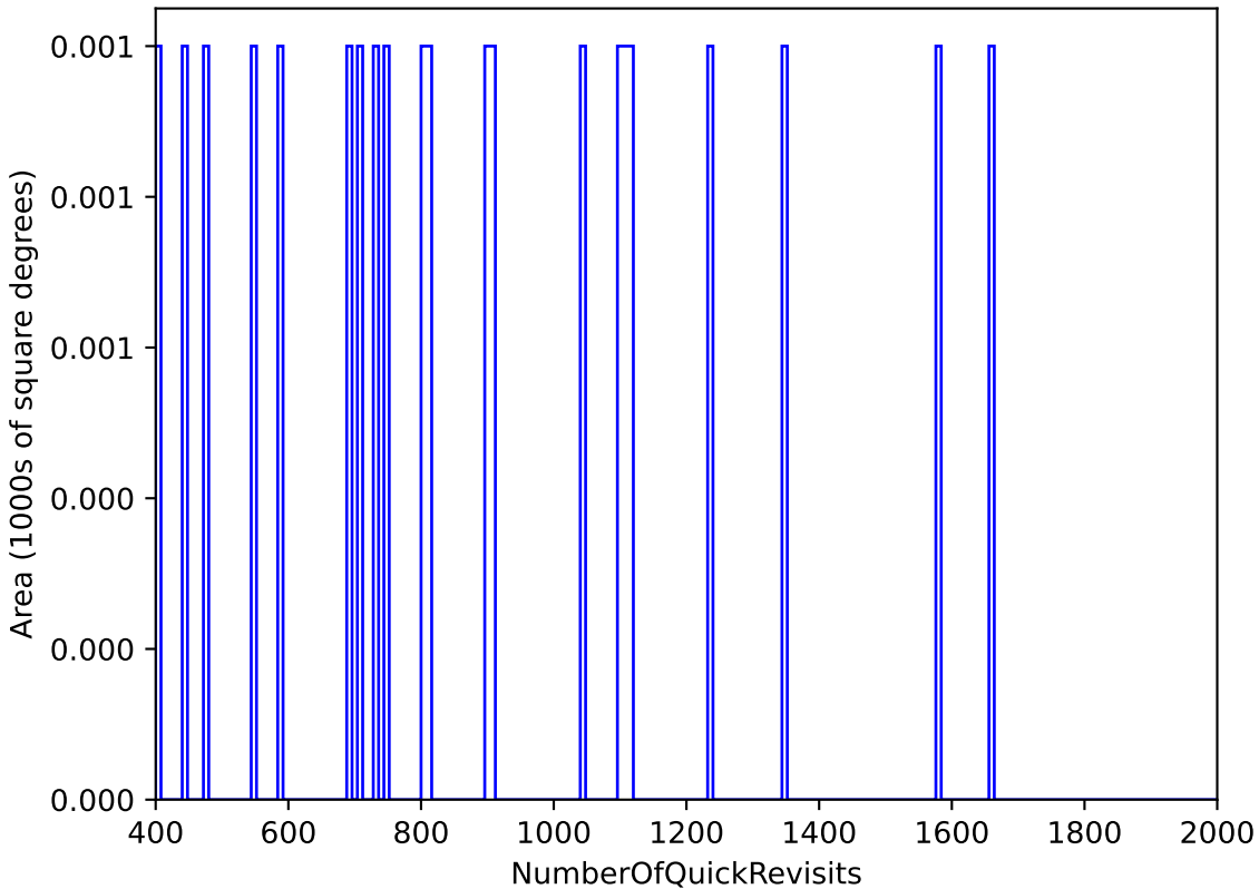
too_elab_heavy_r64_d2_ugrizy_v3.4_10yrs All sky: NumberOfQuickRevisits
