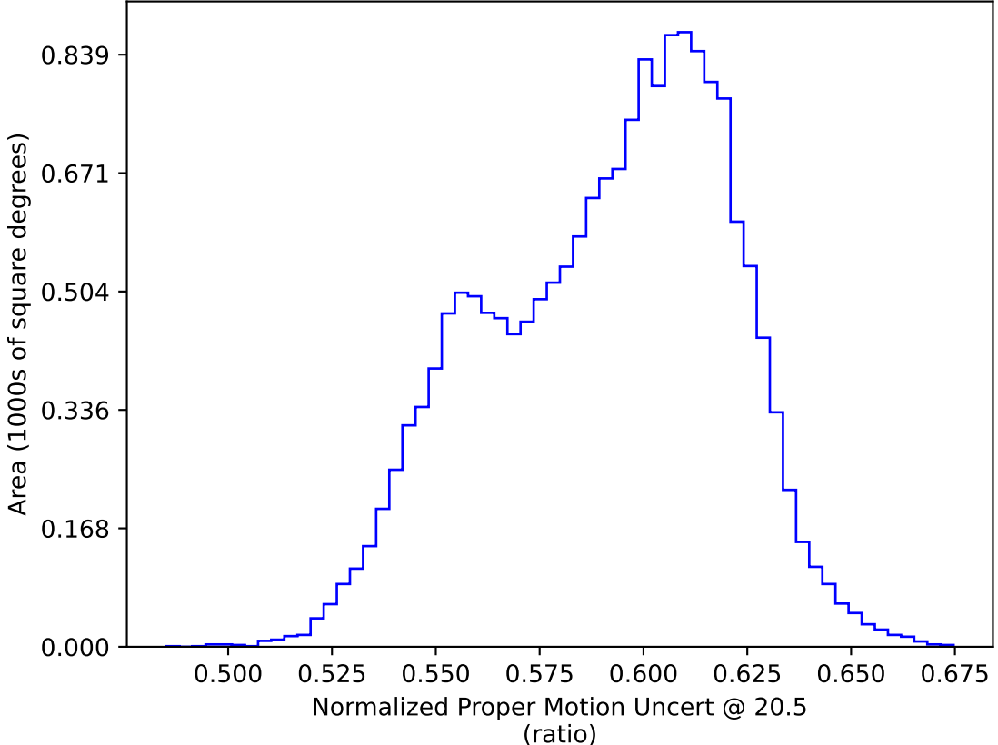
too_elab_heavy_r64_d2_ugrizy_v3.4_10yrs WFD: Normalized Proper Motion Uncert @ 20.5
