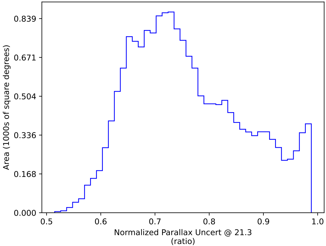
too_elab_heavy_r64_d2_ugrizy_v3.4_10yrs WFD y band only: Normalized Parallax Uncert @ 21.3
