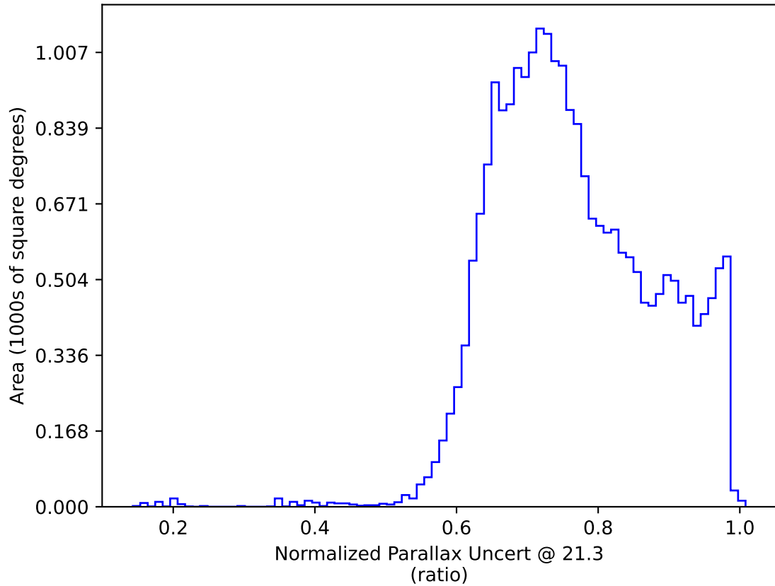
too_elab_heavy_r64_d2_ugrizy_v3.4_10yrs All sky y band only: Normalized Parallax Uncert @ 21.3
