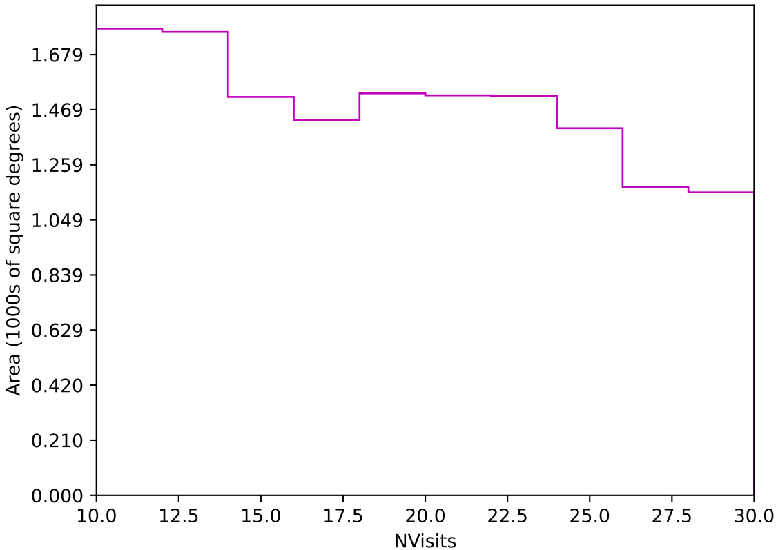
too_elab_heavy_r64_d2_ugrizy_v3.4_10yrs Yr 3-4 z band: NVisits
