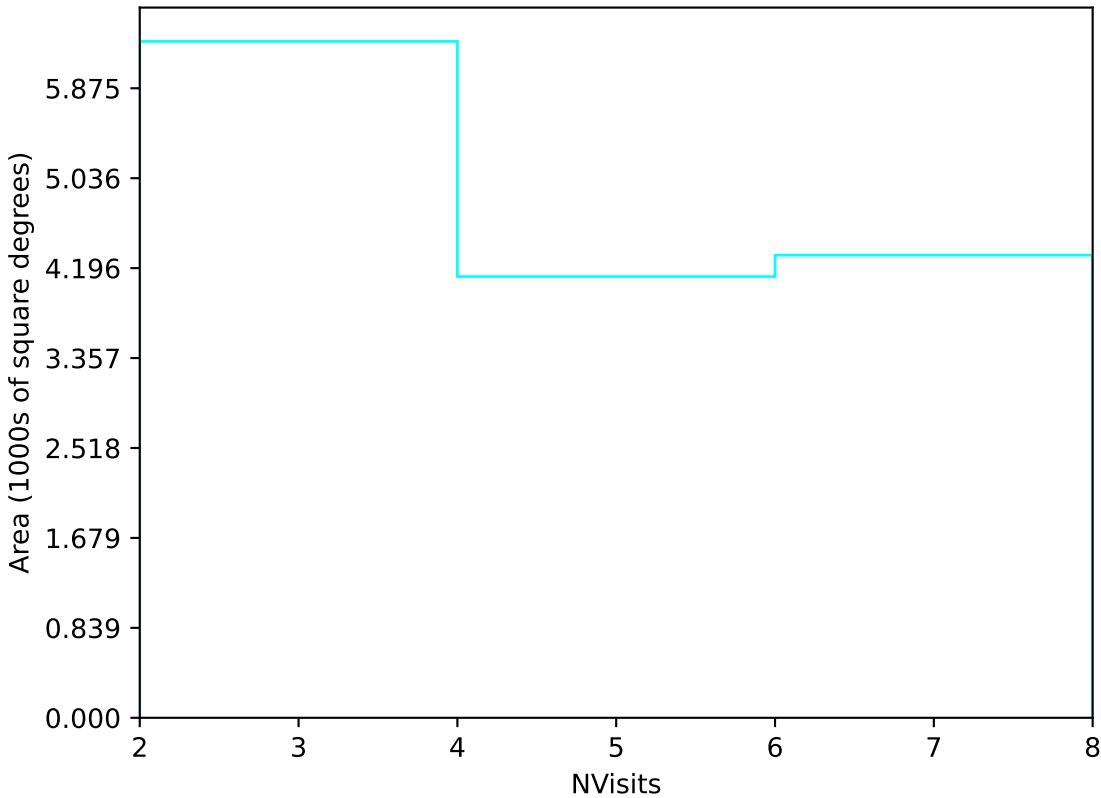
too_elab_heavy_r64_d2_ugrizy_v3.4_10yrs Yr 3-4 u band: NVisits
