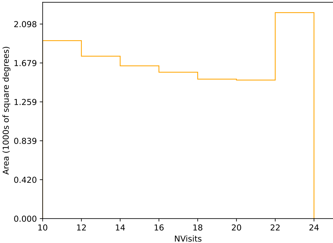
too_elab_heavy_r64_d2_ugrizy_v3.4_10yrs Yr 3-4 r band: NVisits
