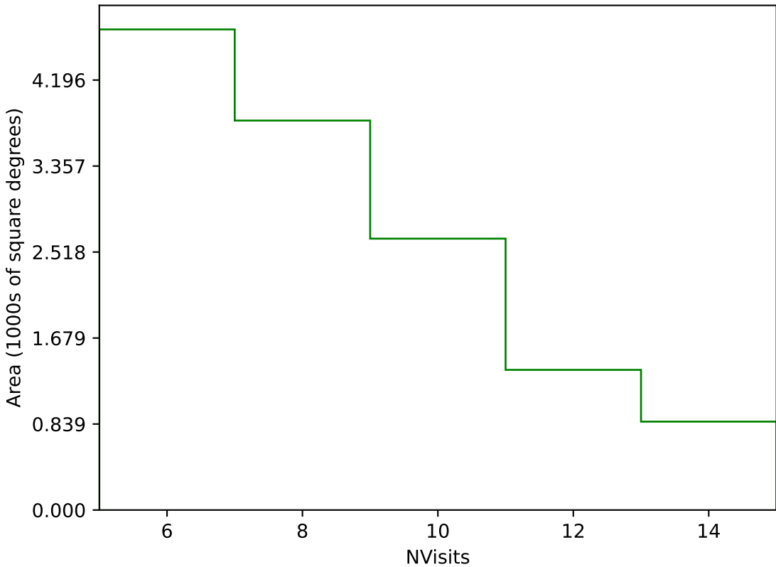
too_elab_heavy_r64_d2_ugrizy_v3.4_10yrs Yr 3-4 g band: NVisits
