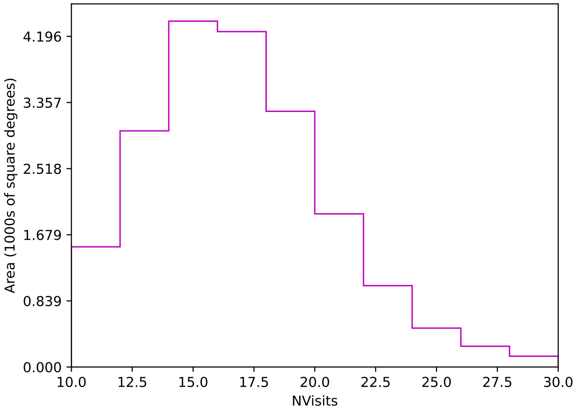
too_elab_heavy_r64_d2_ugrizy_v3.4_10yrs Yr 1 z band: NVisits
