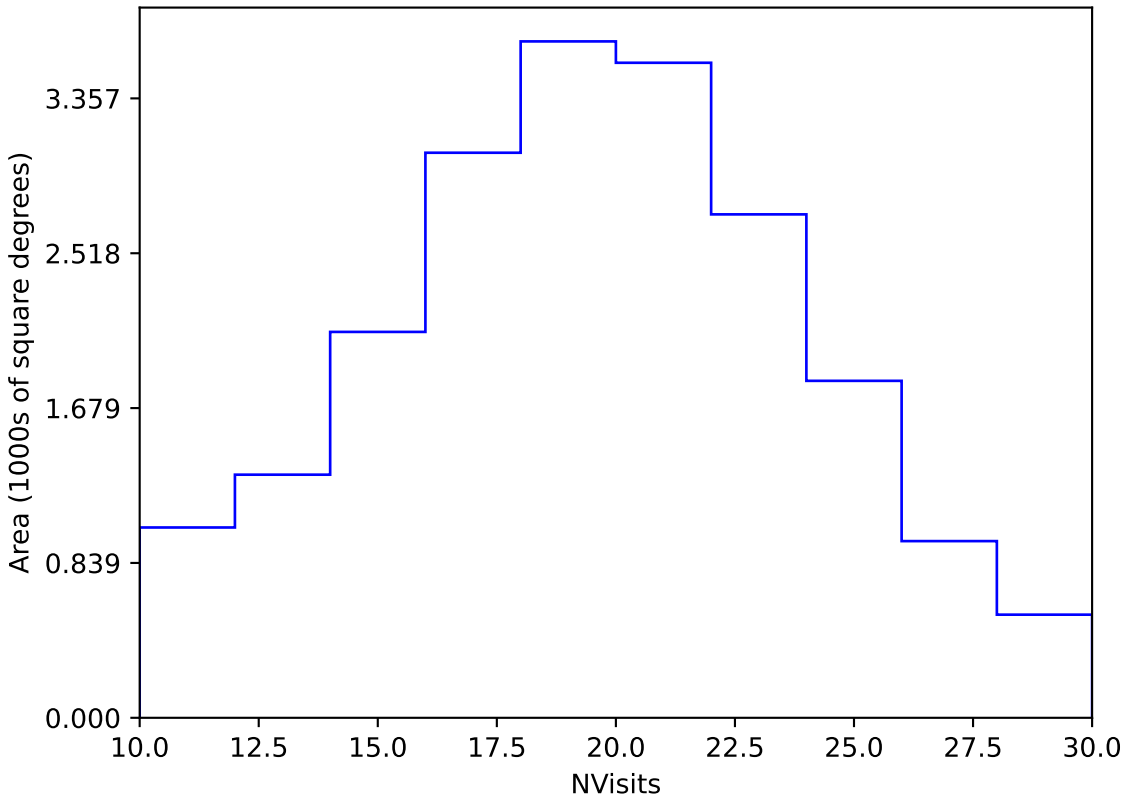
too_elab_heavy_r64_d2_ugrizy_v3.4_10yrs Yr 1 y band: NVisits
