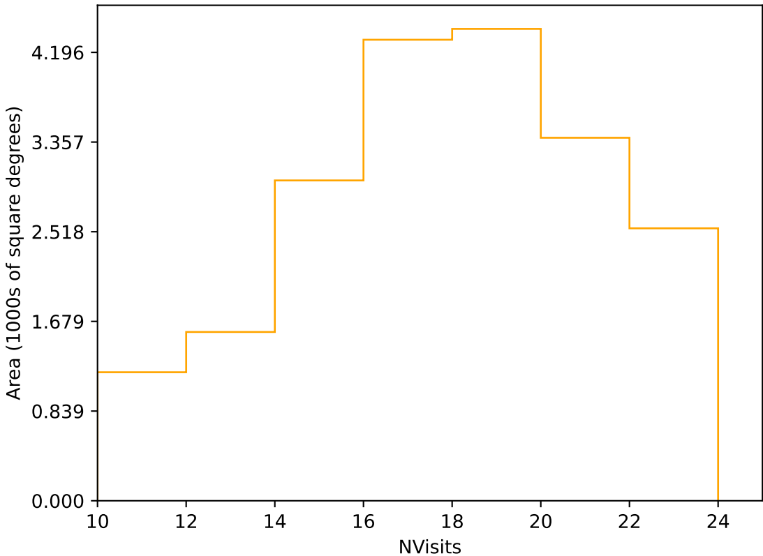
too_elab_heavy_r64_d2_ugrizy_v3.4_10yrs Yr 1 r band: NVisits
