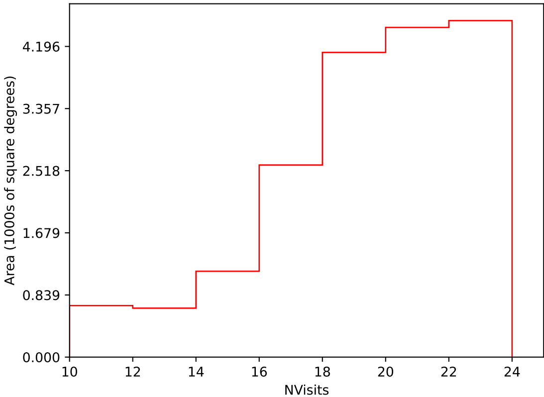
too_elab_heavy_r64_d2_ugrizy_v3.4_10yrs Yr 1 i band: NVisits
