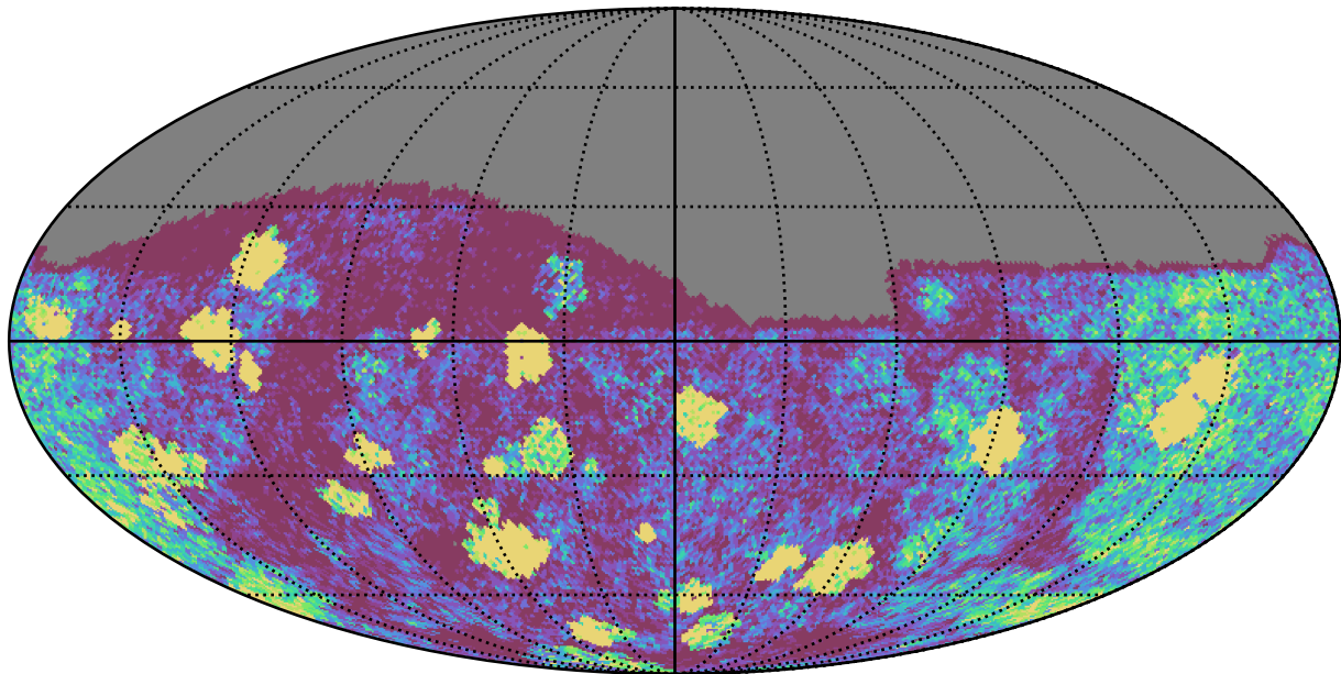
too_elab_heavy_r64_d2_ugrizy_v3.4_10yrs Yr 1 g band: NVisits
