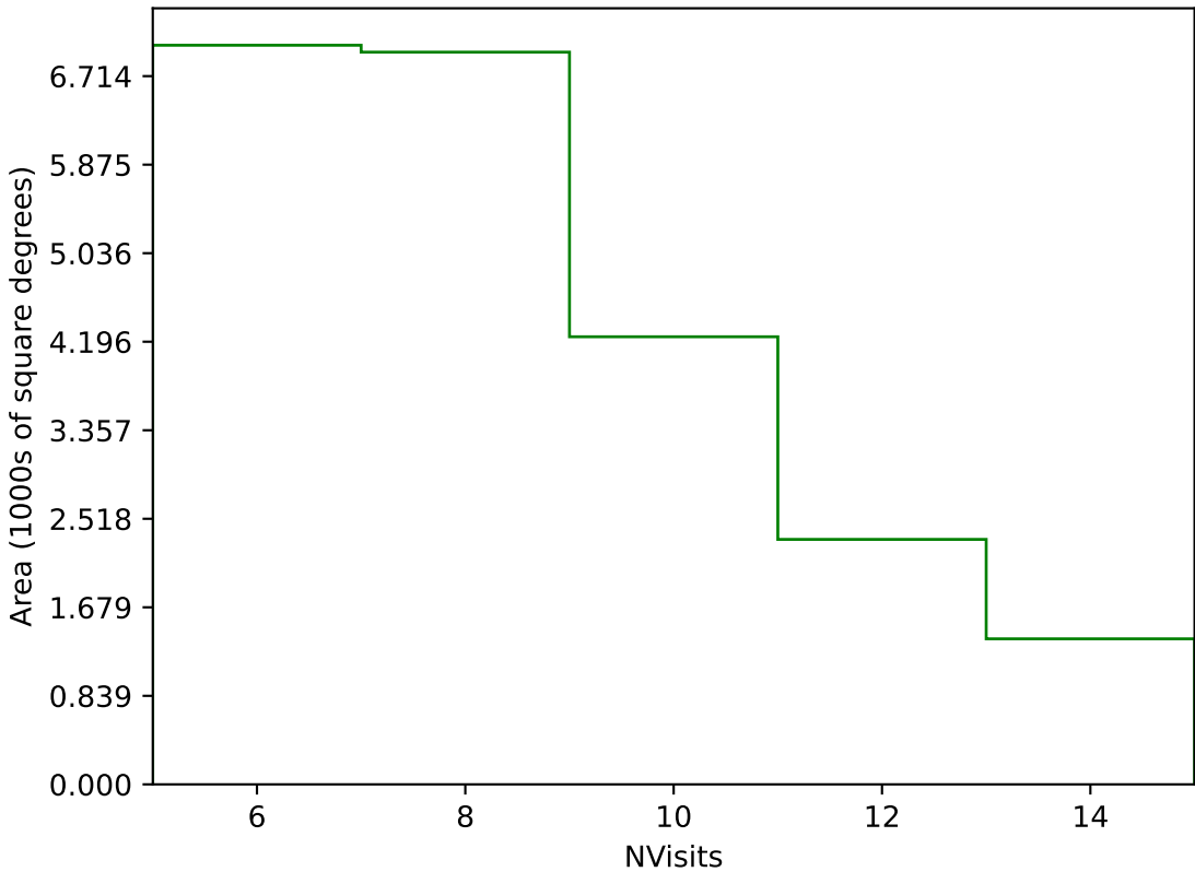
too_elab_heavy_r64_d2_ugrizy_v3.4_10yrs Yr 1 g band: NVisits
