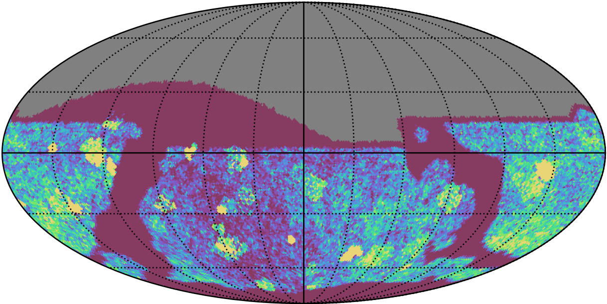
too_elab_heavy_r64_d2_ugrizy_v3.4_10yrs Yr 1 all bands: NVisits
