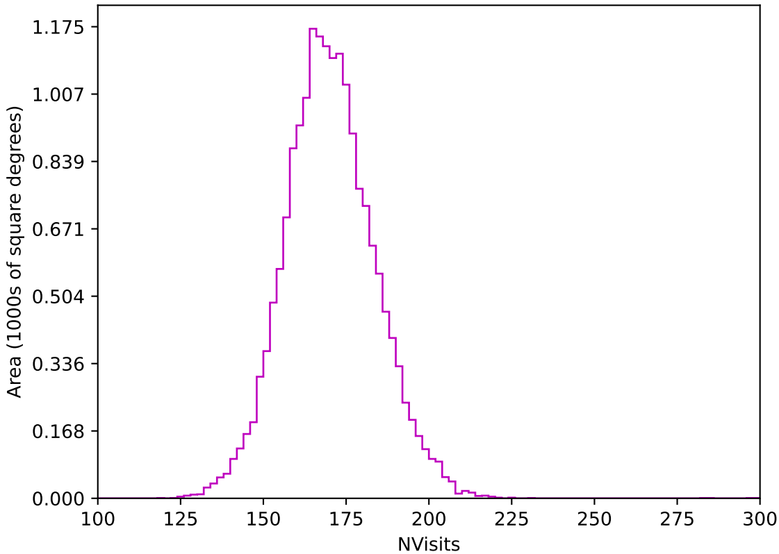
too_elab_heavy_r64_d2_ugrizy_v3.4_10yrs WFD z band: NVisits
