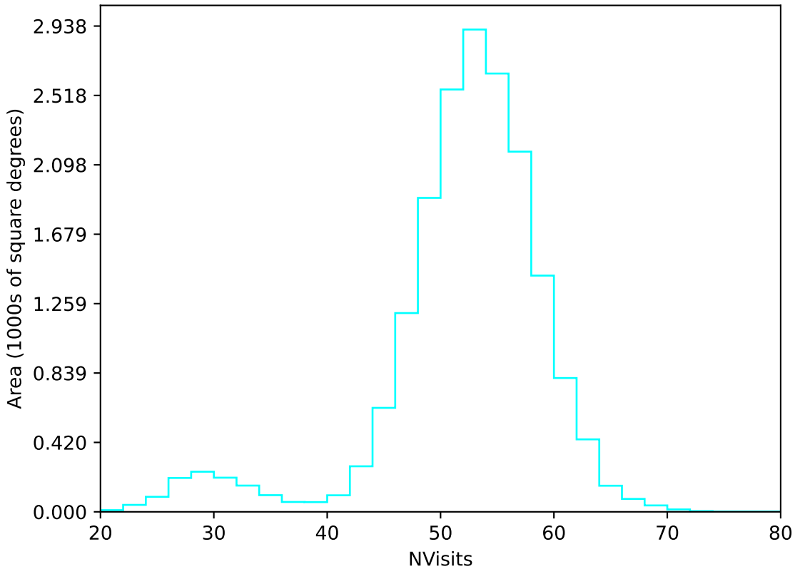
too_elab_heavy_r64_d2_ugrizy_v3.4_10yrs WFD u band: NVisits
