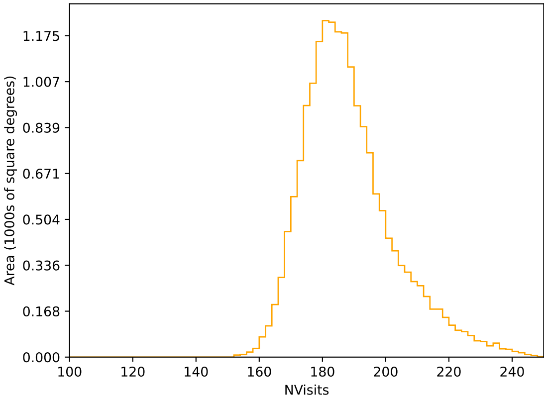
too_elab_heavy_r64_d2_ugrizy_v3.4_10yrs WFD r band: NVisits
