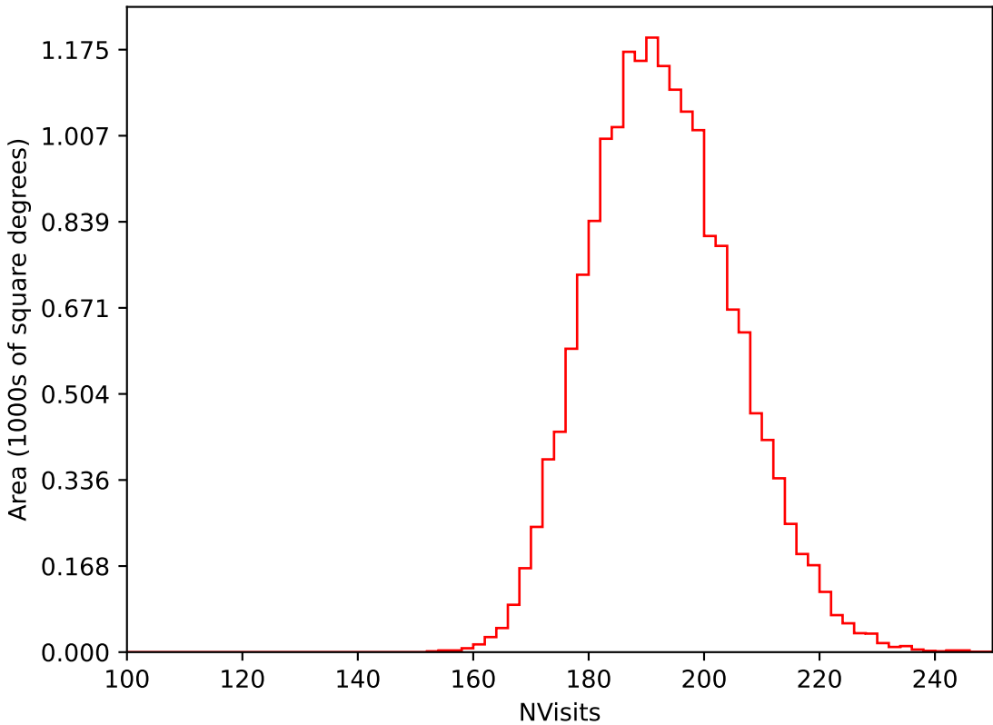
too_elab_heavy_r64_d2_ugrizy_v3.4_10yrs WFD i band: NVisits
