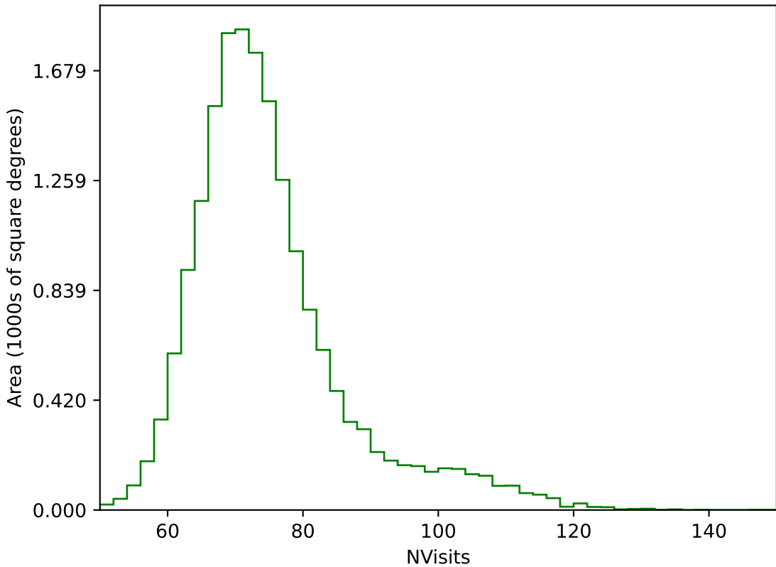
too_elab_heavy_r64_d2_ugrizy_v3.4_10yrs WFD g band: NVisits
