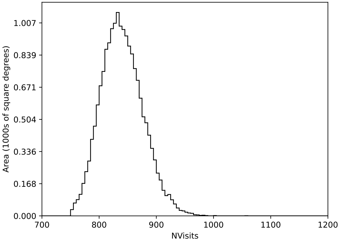
too_elab_heavy_r64_d2_ugrizy_v3.4_10yrs WFD all bands: NVisits
