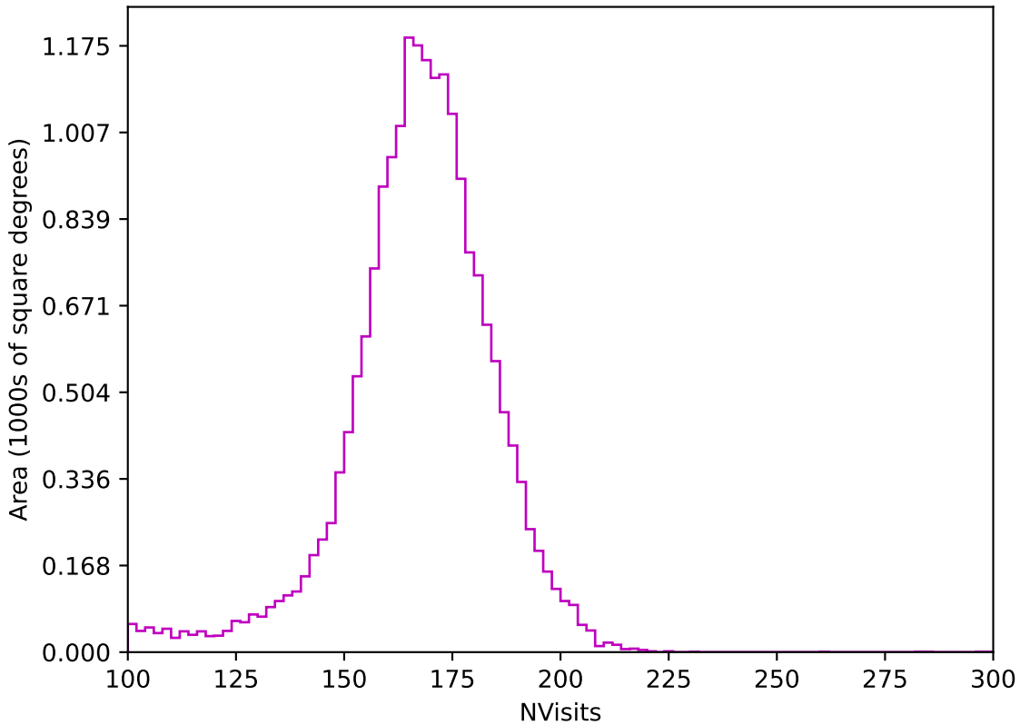
too_elab_heavy_r64_d2_ugrizy_v3.4_10yrs All sky z band: NVisits
