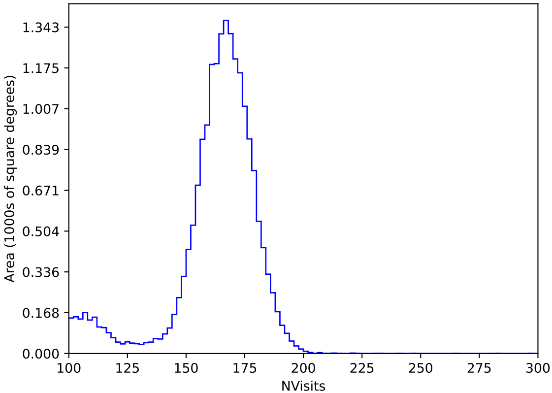
too_elab_heavy_r64_d2_ugrizy_v3.4_10yrs All sky y band: NVisits
