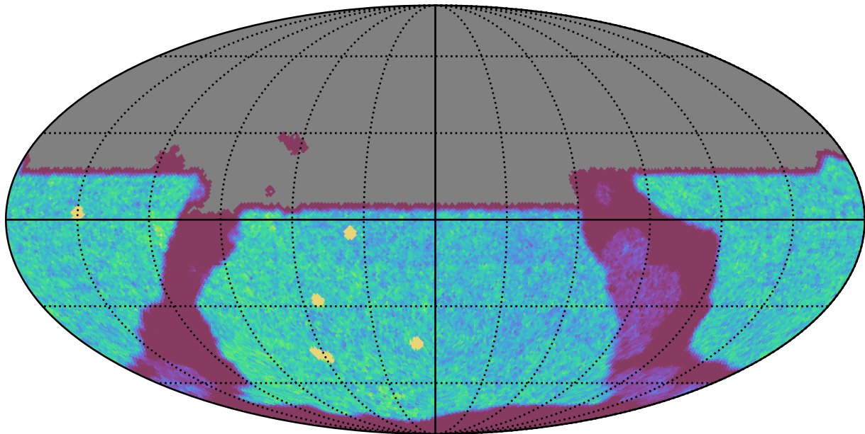
too_elab_heavy_r64_d2_ugrizy_v3.4_10yrs All sky u band: NVisits
