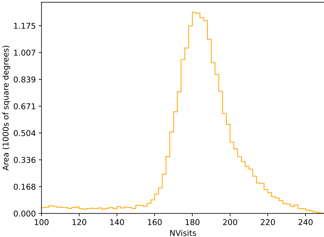
too_elab_heavy_r64_d2_ugrizy_v3.4_10yrs All sky r band: NVisits
