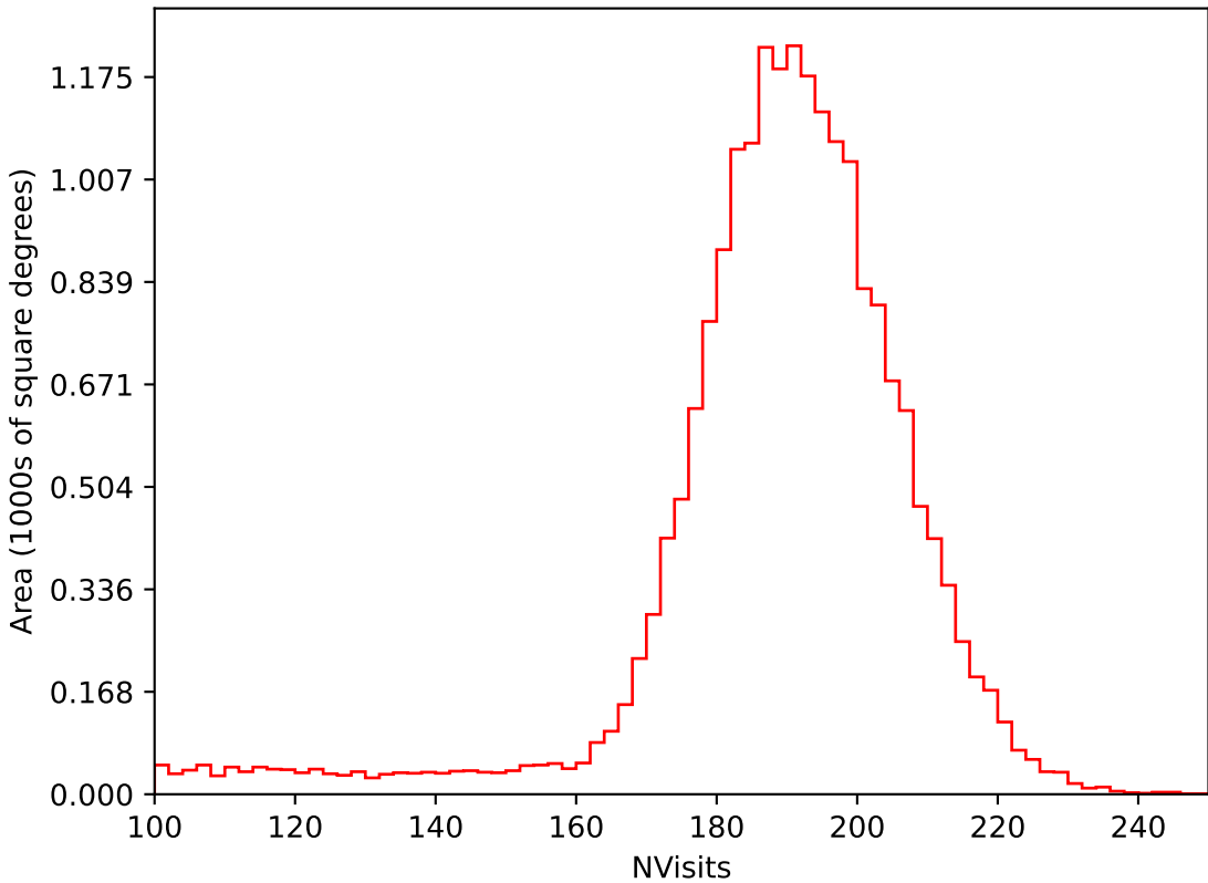
too_elab_heavy_r64_d2_ugrizy_v3.4_10yrs All sky i band: NVisits
