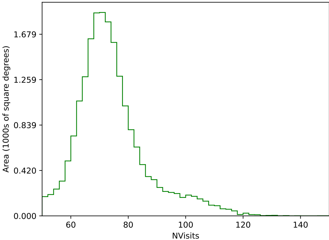
too_elab_heavy_r64_d2_ugrizy_v3.4_10yrs All sky g band: NVisits
