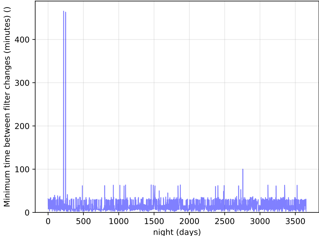
too_elab_heavy_r64_d2_ugrizy_v3.4_10yrs Per Night: Minimum time between filter changes (minutes)
