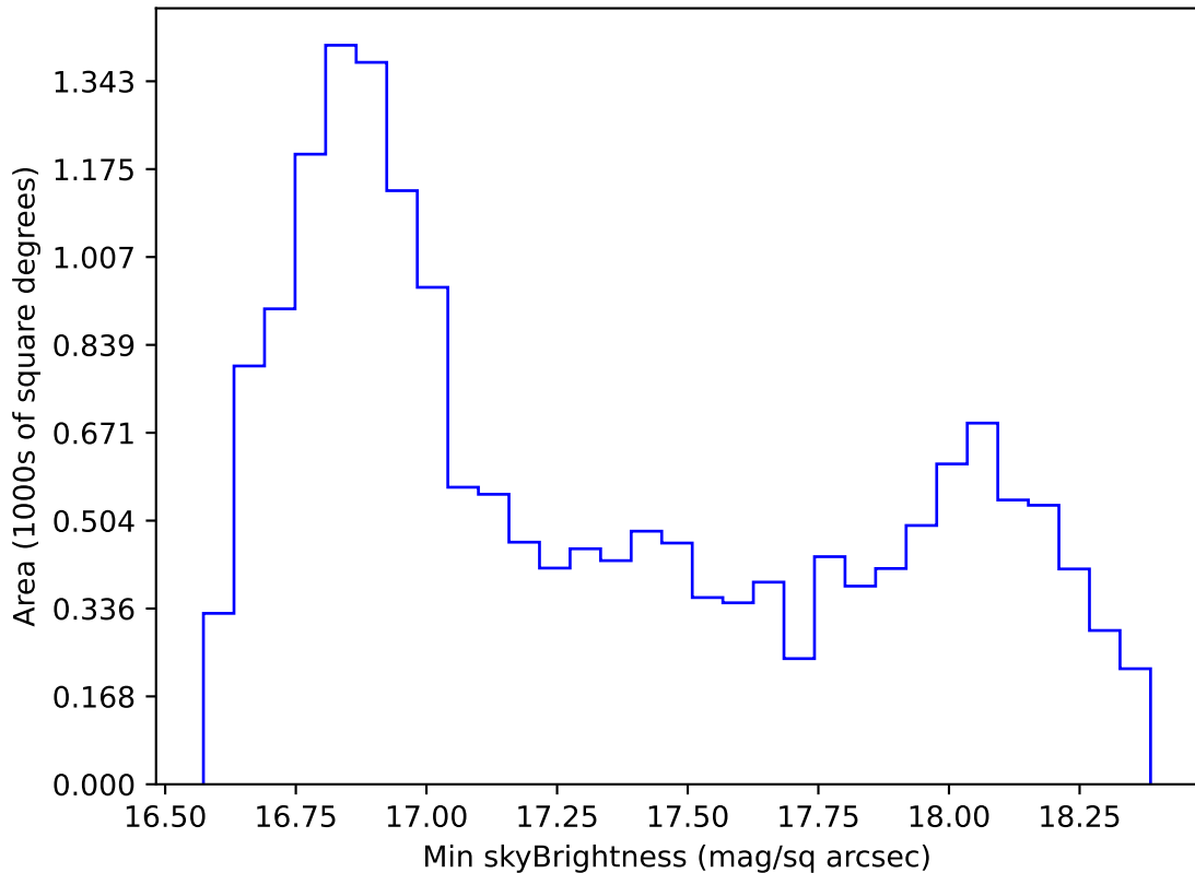
too_elab_heavy_r64_d2_ugrizy_v3.4_10yrs WFD z band: Min skyBrightness
